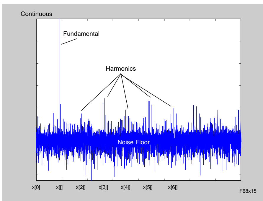
- Figure 15. FFT -
