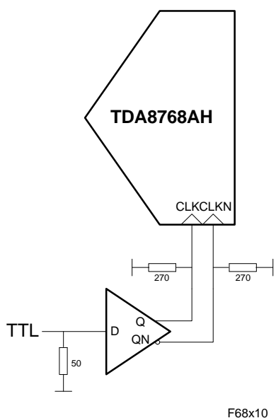
- Figure 10: Example of TTL/PECL interface -
