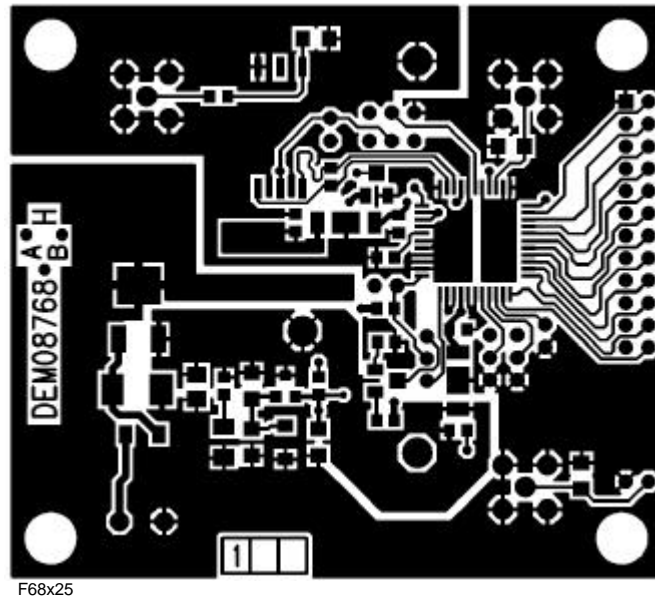
- Figure 28. Topside component layout (signal layer 1) -
